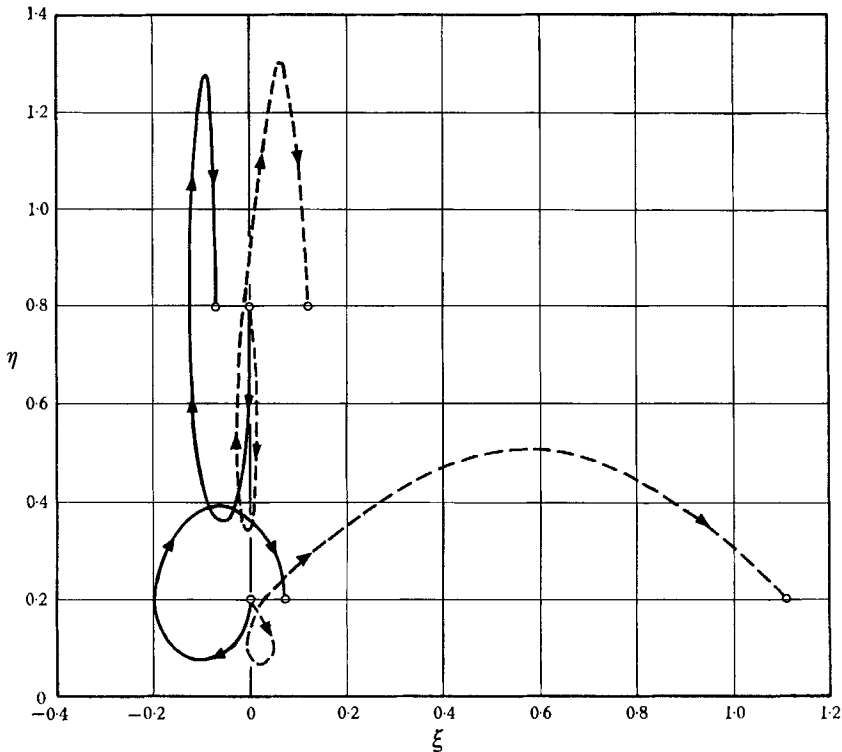
FIGURE 9. Samples of particle trajectories for the plane case, with \phi = \frac{1}{2} : two-dimensional; sine wave; particle orbits for \eta_0 = 0.2 , \eta_0 = 0.8 at \tau = 0 and \xi = 0 . ———, \theta/\theta_0 = 0 ; - - - - -, \theta/\theta_0 = 1 .
